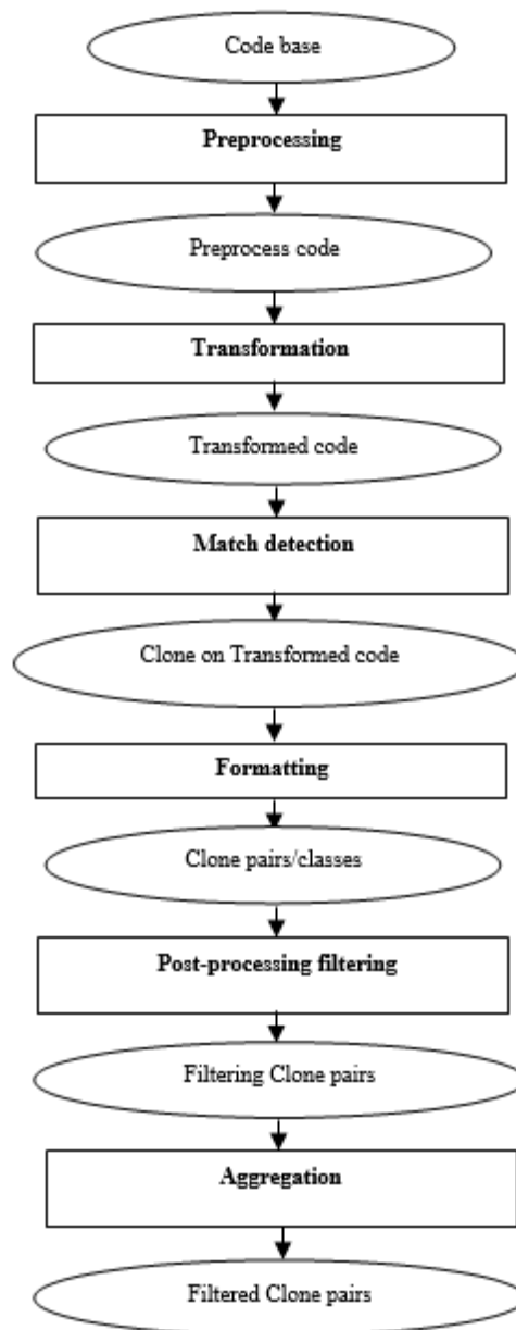
Fig.1: Generic Clone Detection Process
